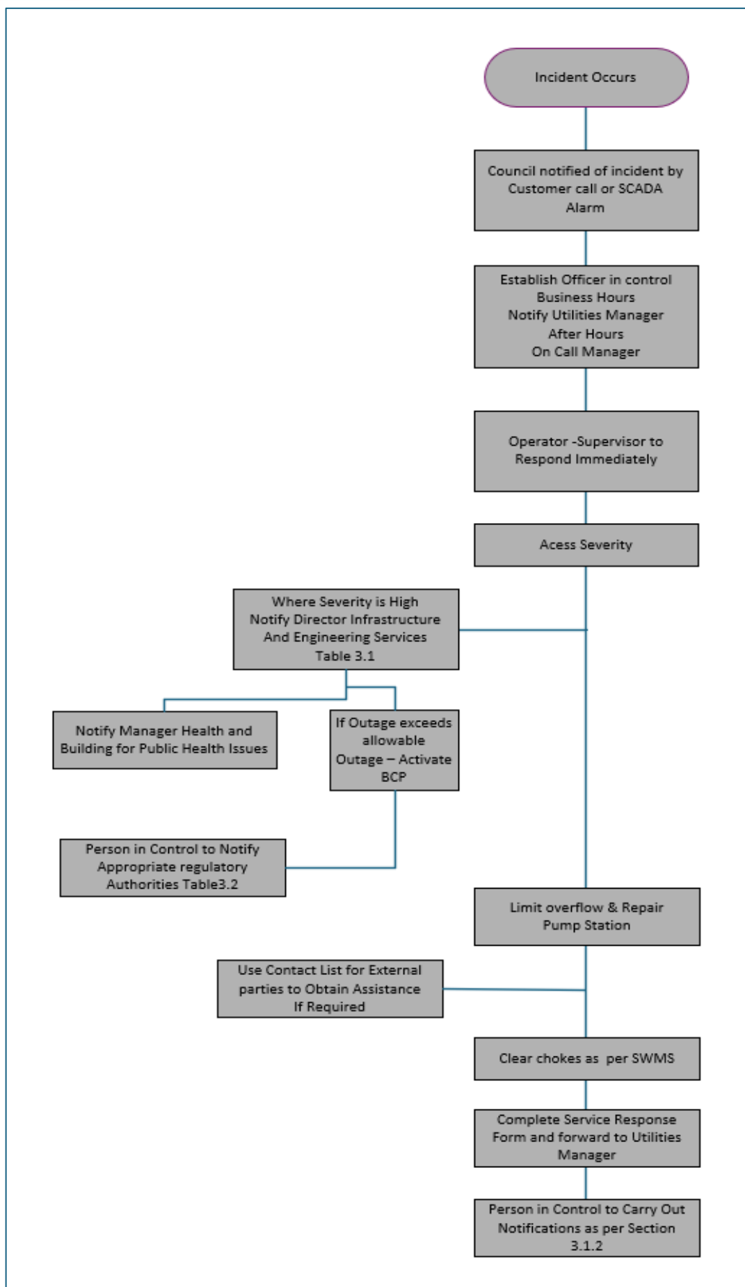
Figure 3.2 Incident Response Flowchart Overflow or Spill
